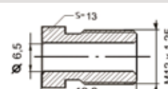
Union steel male M12x1,25/Ø6,5mm
