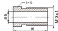
Union steel male M10x1,0/Ø5mm
