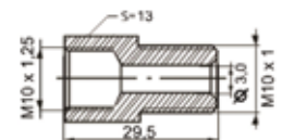
Reducer female M10x1,25-male M10x1,0
