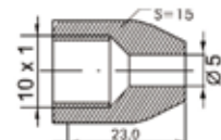
Union steel female 3/8"unf / Ø5mm
