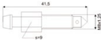
Bleedvalve M8x1,25 L=41,5mm
