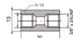
Coupler female Brass 3/8"unf convex
