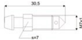
Bleedvalve M7x1 L=30,5mm
