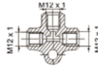
T-stuk Brass 3x M12x1,0 convex
