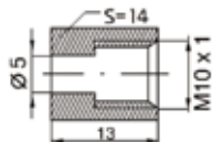
Union steel female M10x1,0/Ø5mm
