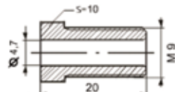
Union steel male M9 / Ø4,7mm
