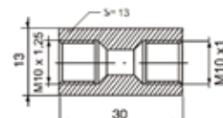
Fem. Reducer M10x1,25 - M10x1,0 convex
