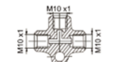
T-stuk Brass 3x M10x1,0 concave
