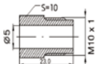
Union steel male M10x1,0 / Ø5mm
