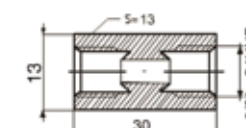
Coupler female Brass 3/8"unf concave
