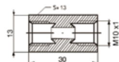
Coupler female Brass M10x1,0 concave
