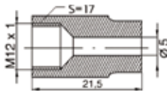
Union steel female M12x1,0/Ø5mm
