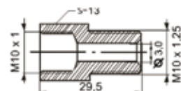
Reducer female M10x1,0-male M10x1,25
