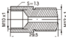
Reducer female M10x1,0-male M12x1,0
