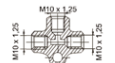
T-stuk Brass 3x M10x1,25 convex
