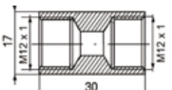
Coupler female Brass M12x1,0 convex
