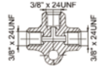
T-stuk Brass 3x 3/8"unf concave
