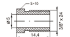
Union steel male 3/8"unf / Ø5mm
