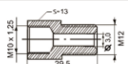
Reducer female M10x1,25-male M12x1,0
