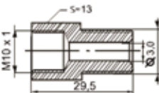
Reducer female M10x1,0-male M10x1,0
