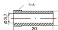
Union steel male M8 / Ø3,7mm
