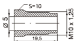
Union steel male M10x1,25/Ø5mm
