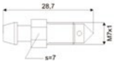
Bleedvalve M7x1 L=28,7mm
