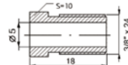
Union steel male 3/8"unf / Ø5mm
