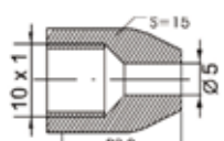
Union steel female M10x1,0/Ø5mm
