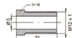
Union steel male M12x1,0/Ø5mm
