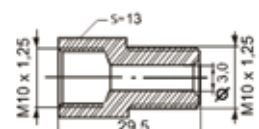
Reducer female M10x1,25-male M10x1,25
