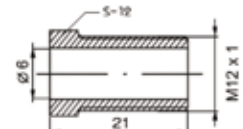
Union steel male M12x1,0/Ø6mm
