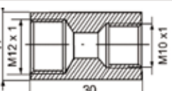
Female Reducer M12x1,0-M10x1,0 convex
