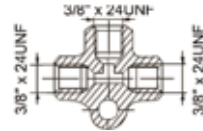
T-stuk Brass 3x 3/8"unf convex
