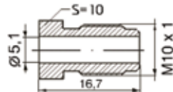
Union steel male M10x1,0/Ø5,1mm
